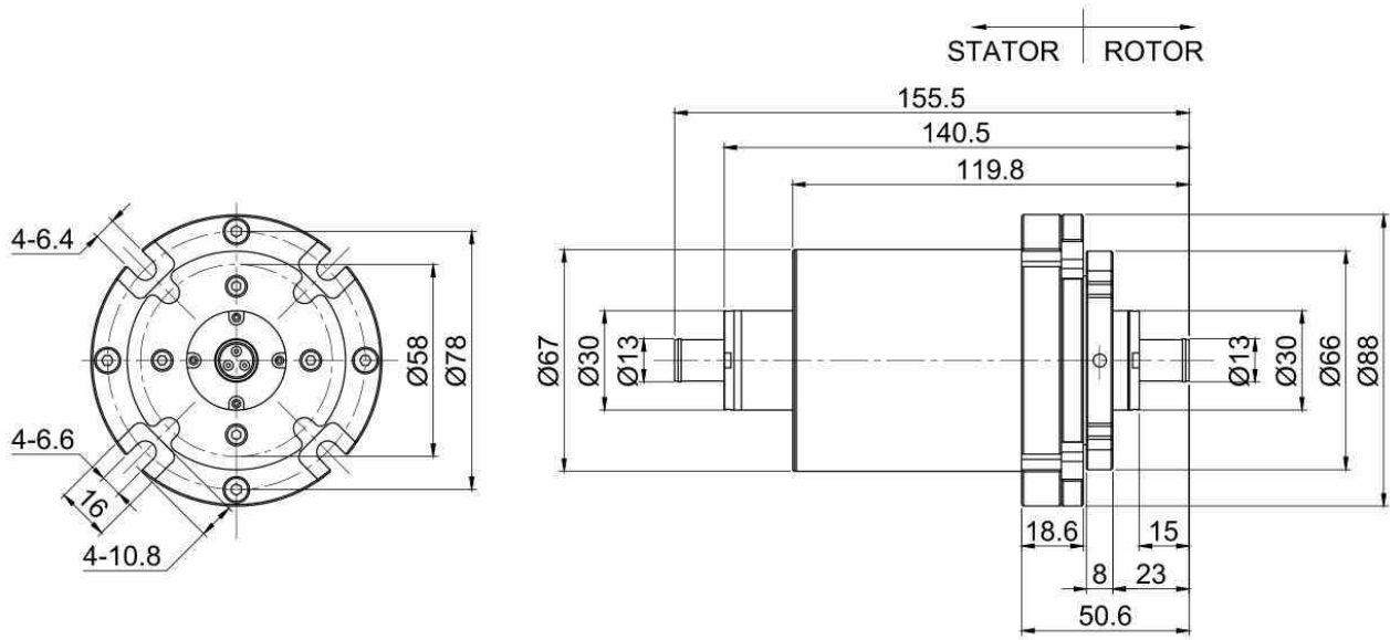
Drawing for CHG067A-N
